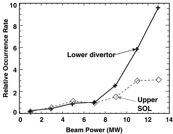
Fig. 5. The occurrence rate for inject power at the time of a dust event, binned over 2 MW, normalized the occurrence rate over all times searched for the lower divertor (pluses) and the upper SOL (diamonds).
