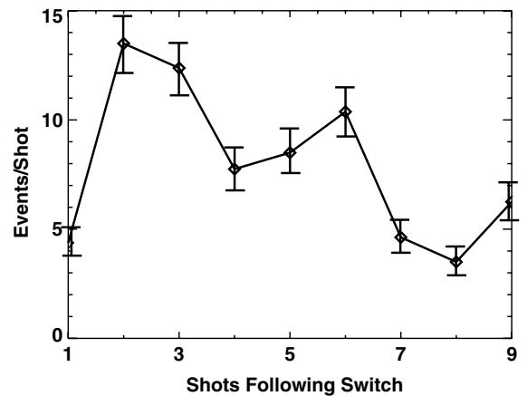
Fig. 6. The number of dust events per shot in the upper SOL as a function of the number of shots following a switch from a period of LN dominant operation to a period of UN dominance, averaged over the eight switches that occurred during the 9 months of data accumulation. The average rate over all UN dominant shots is 3.4 events/shot.
