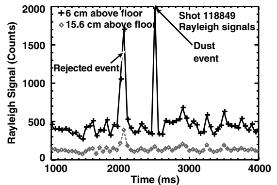
Fig. 2. The Rayleigh channel signal as a function of time is shown for two spatial channels for the plasma shown in Fig. 1. The event at 2500 ms is recorded as a dust event, but the event just after 2000 ms is rejected because it was observed in several spatial channels simultaneously.
