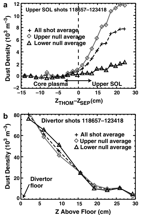
Fig. 4. The density of dust particles as a function of distance along the laser path for (a) the upper SOL (density is referenced to the average location of the separatrix over all times searched) and (b) the lower divertor (distance is referenced to the divertor strike plate).
