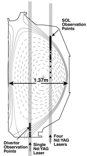
Fig. 1. The DIII-D Thomson laser paths and viewing volumes for the upper SOL and lower divertor are shown along with a flux surface plot of a lower single-null plasma. There are four collinear lasers passing along the path through the upper SOL, only one passes through the divertor. Laser beam width, nominally \sim 3 mm, and observation volumes are not to scale.
