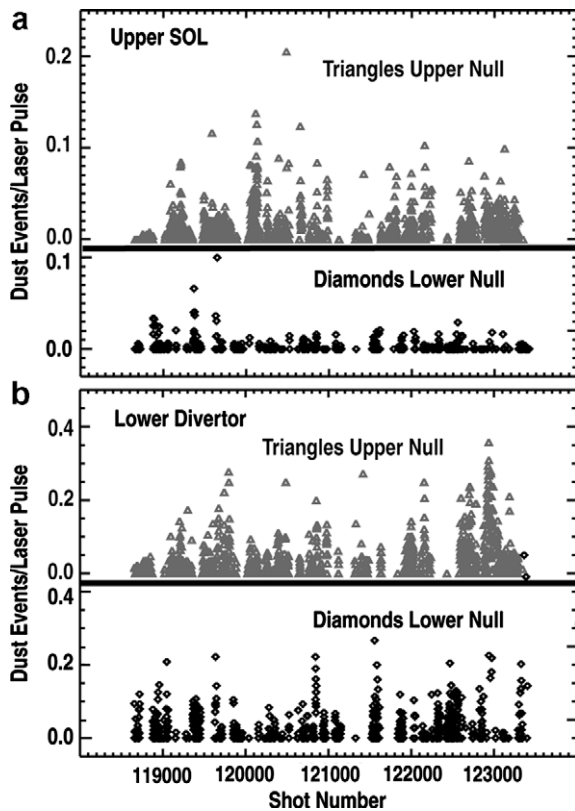
Fig. 3. Histograms of the number of dust events per laser pulse for all spatial channels as a function of shot number in the (a) upper SOL region, and (b) lower divertor region over the span of 9 months of operation on DIII-D. The upper curves (gray triangles) are for UN dominant shots, the lower curves (black diamonds) are for LN dominance.
